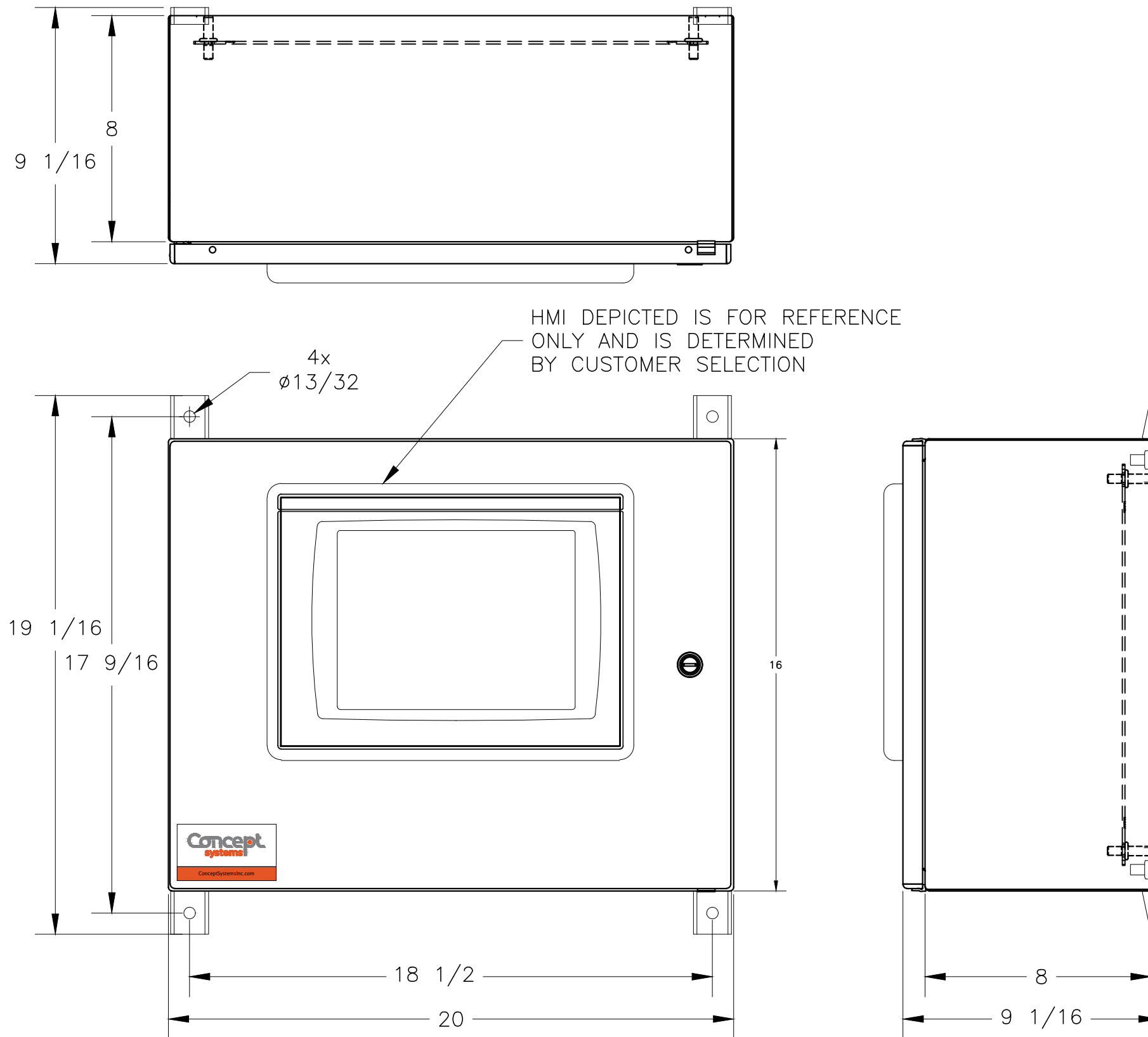
WALL MOUNT ENCLOSURE DIMENSIONS
