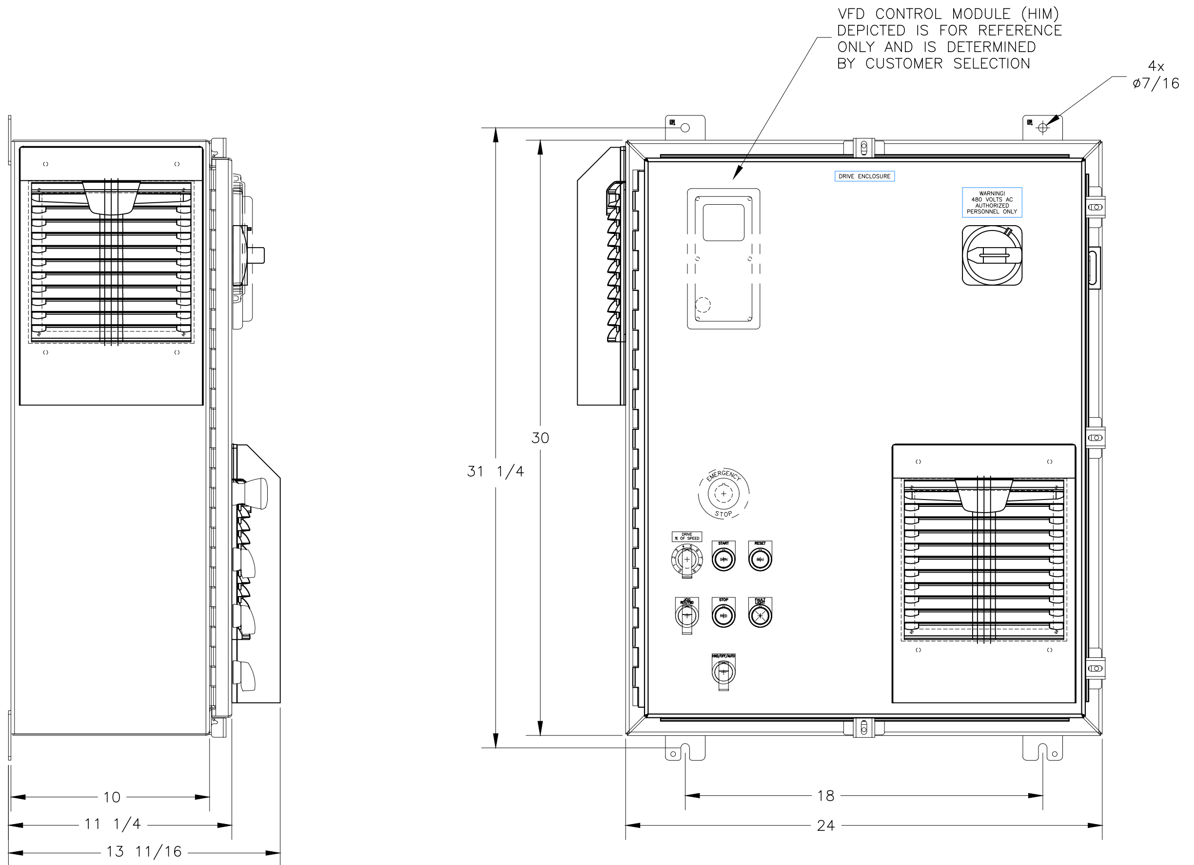
0.5 TO 3 HP VFD UL TYPE 4X ENCLOSURE DIMENSIONS
