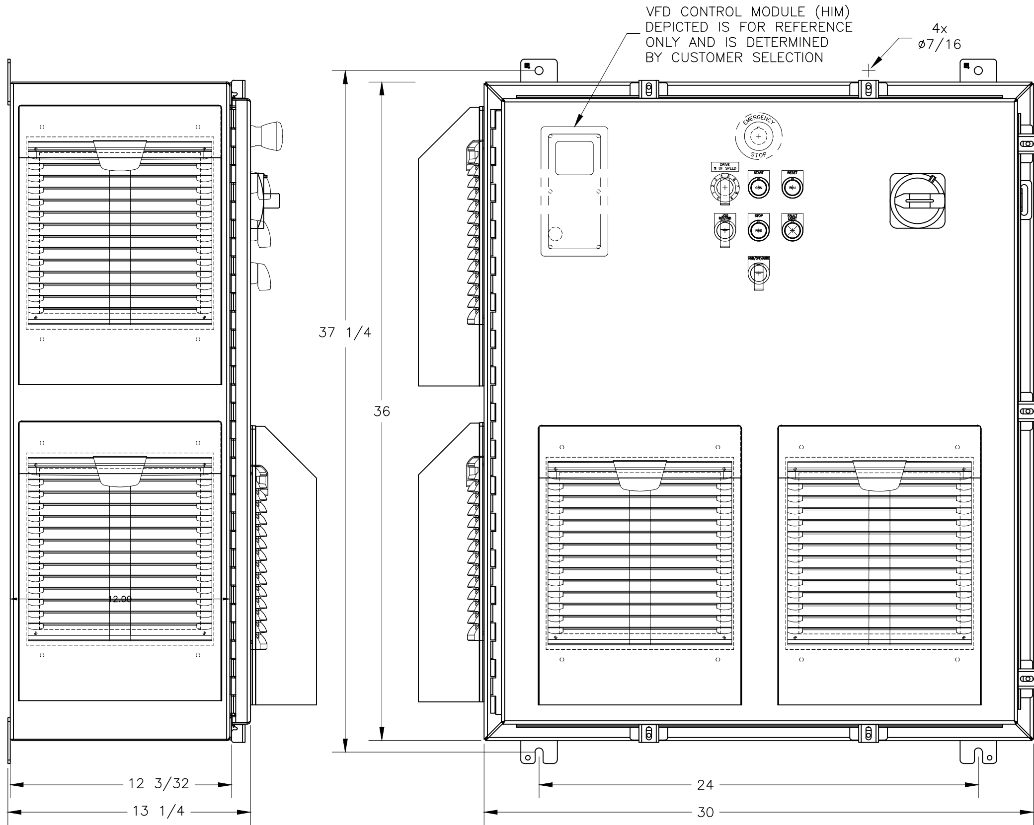
10 TO 20 HP VFD UL TYPE 4X ENCLOSURE DIMENSIONS
