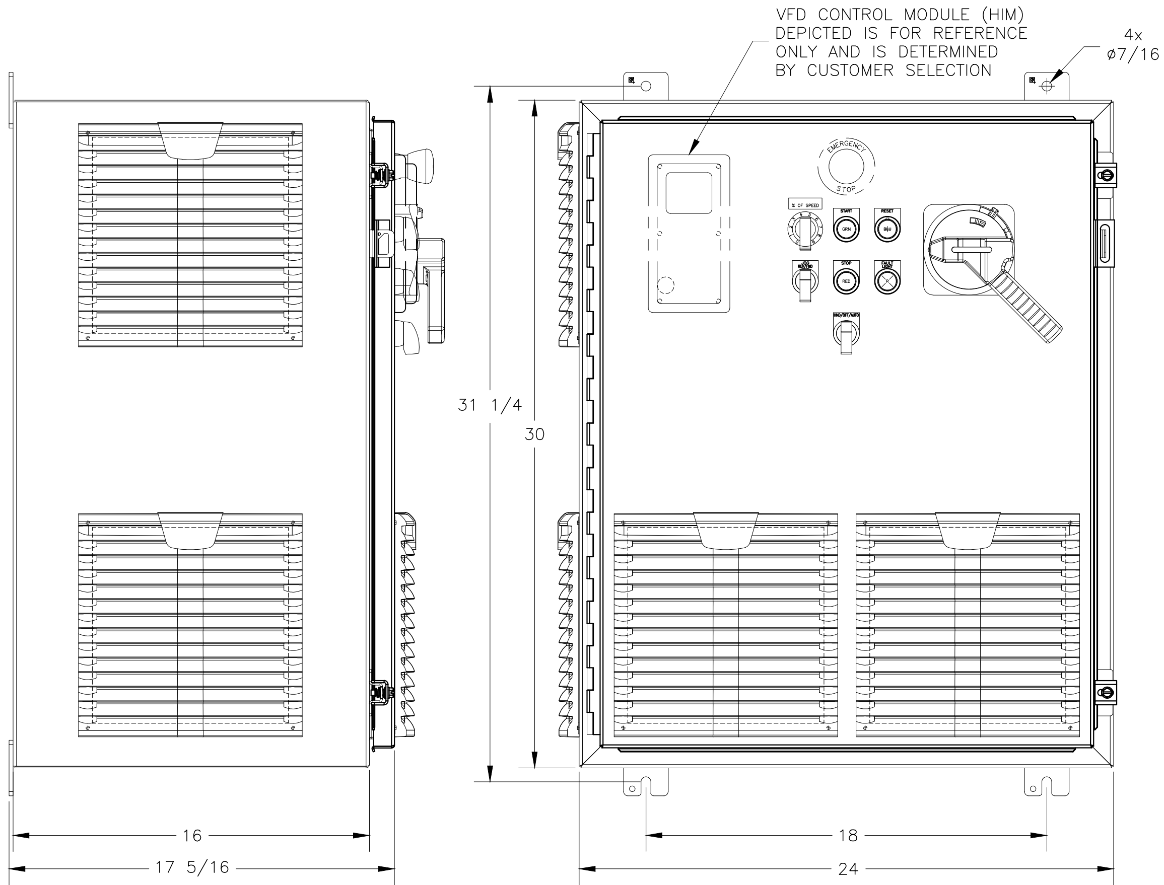
25 TO 30 HP VFD ENCLOSURE DIMENSIONS
