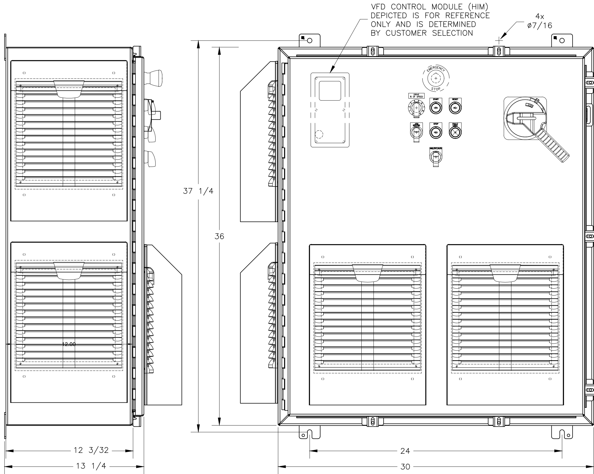
25 TO 30 HP VFD UL TYPE 4X ENCLOSURE DIMENSIONS
