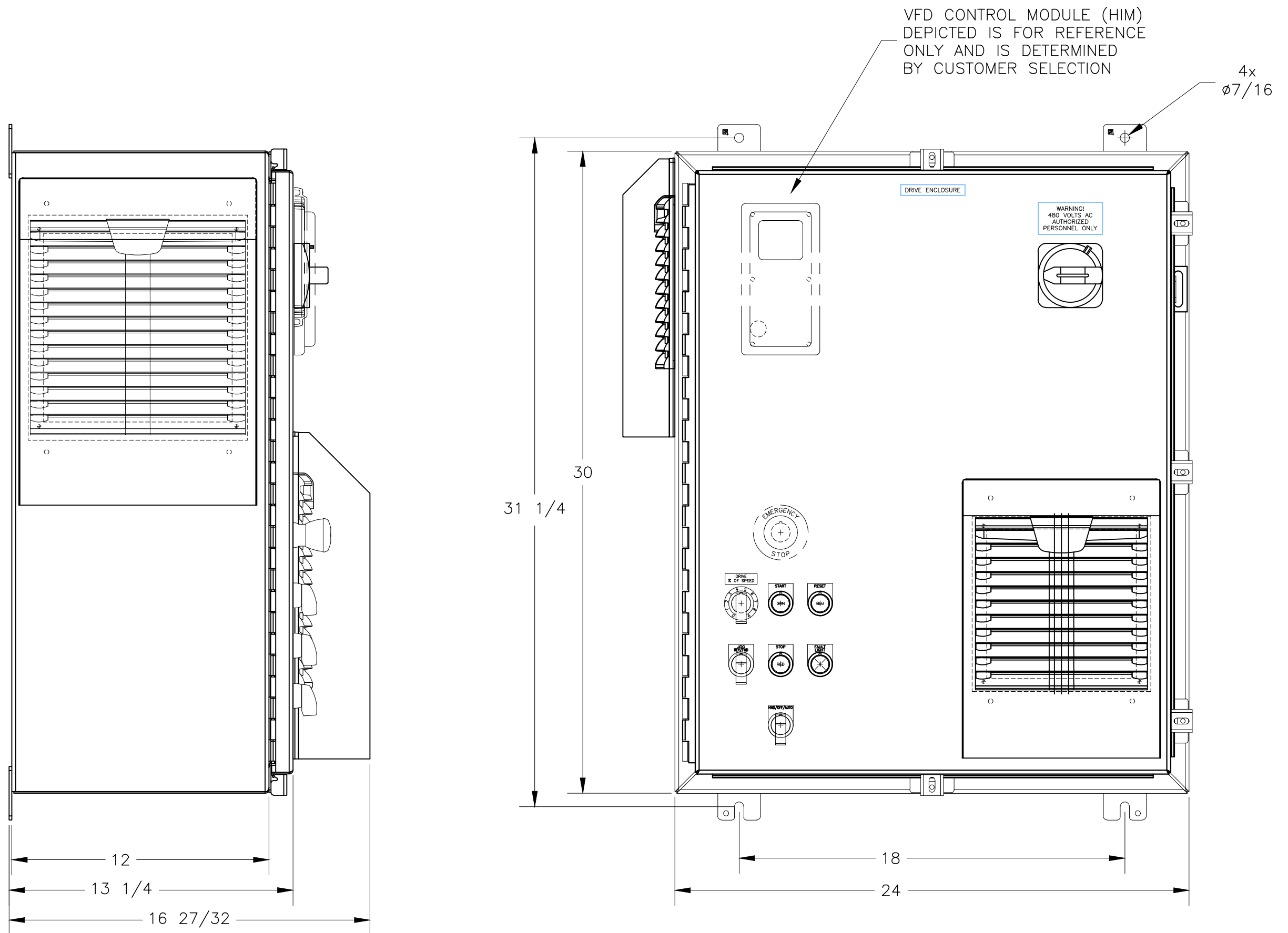
5 HP VFD UL TYPE 4X ENCLOSURE DIMENSIONS
