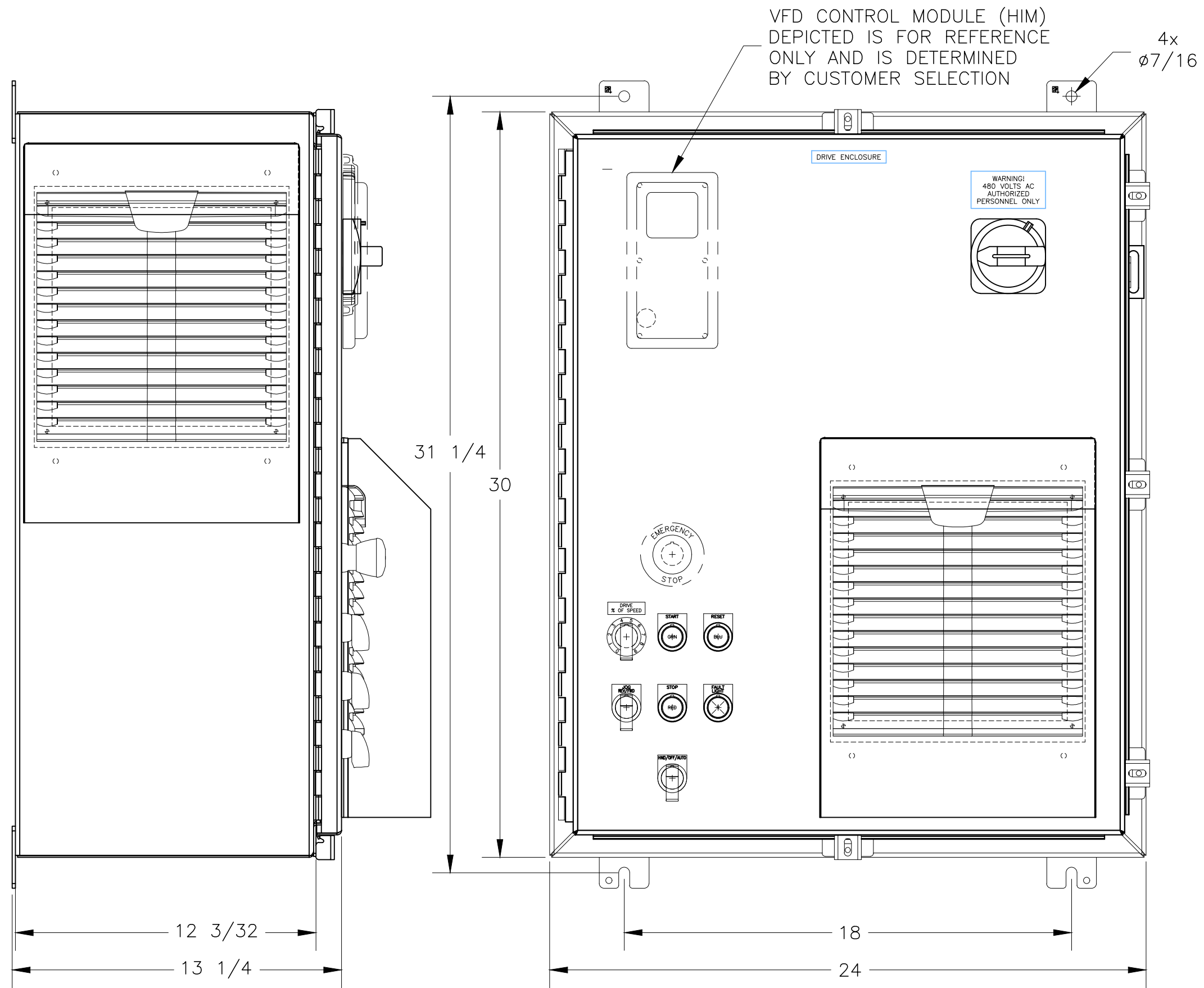
7.5 HP VFD UL TYPE 4X ENCLOSURE DIMENSIONS
